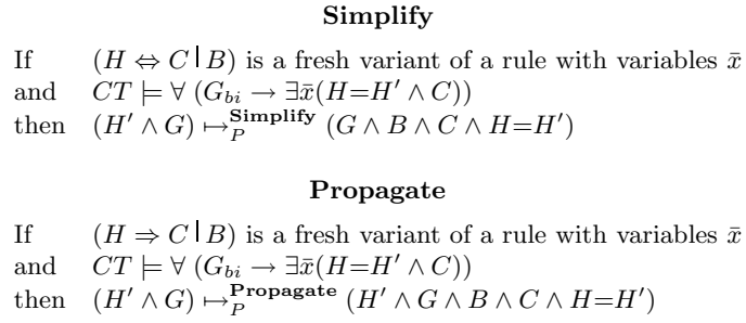
Fig. 1. Computation Steps of Constraint Handling Rules
